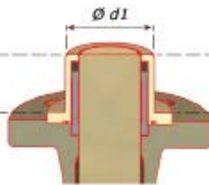
Type 28KR Soft seal in the vessel
