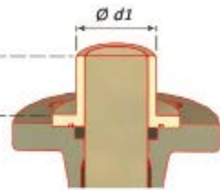
Type 28KV-E Soft seal in the valve body with extended sleeve
