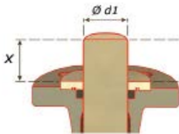
Type 28KV Soft seal in the valve body
