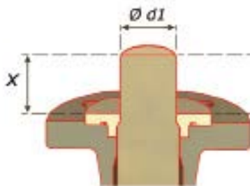
Type 28KX Metal seal in the valve body
