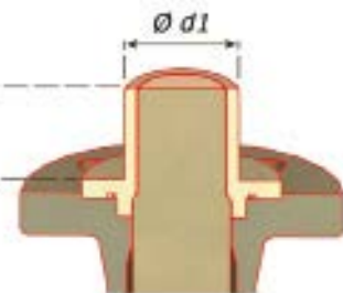
Type 28KX-E Metal seal in the valve body with extended sleeve
